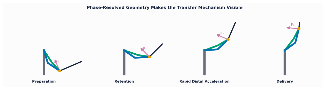
Figure 23.1: Phase-Resolved Geometry of the Advanced Model
