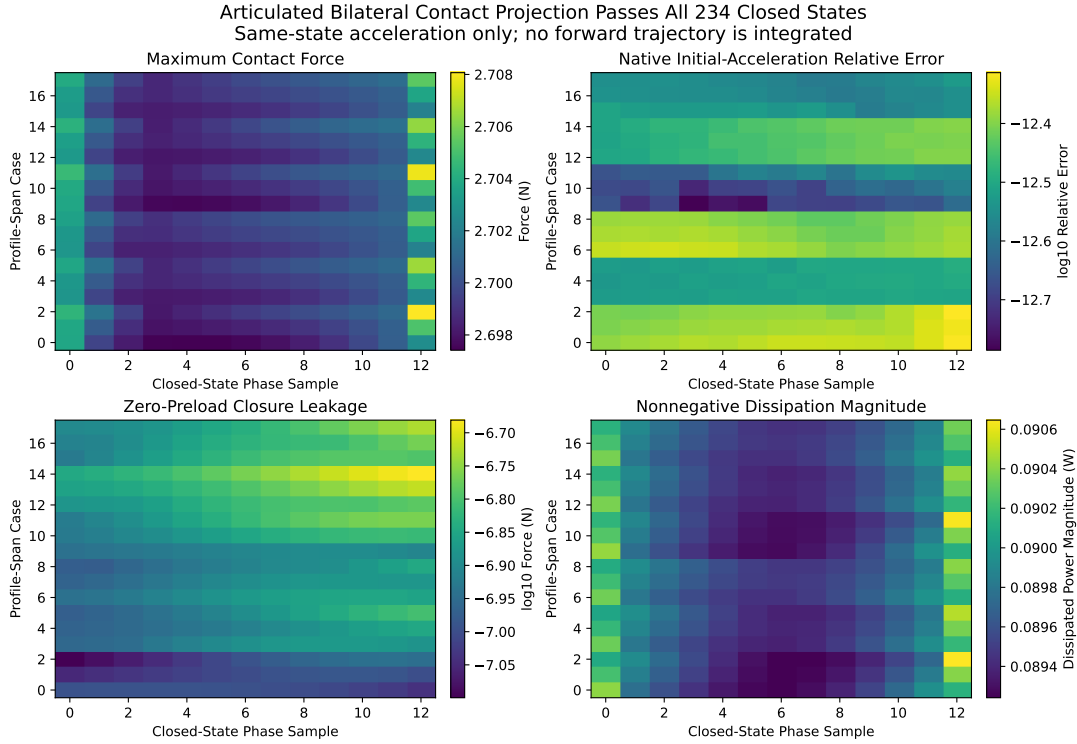
Figure 17.10: Articulated Contact Projection and Initial Acceleration Across All Closed States
