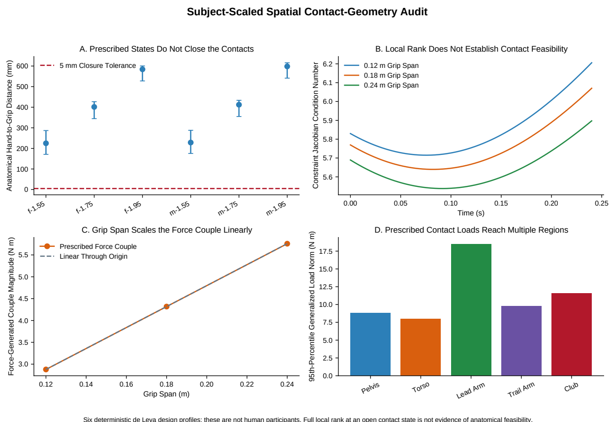
Figure 17.4: Subject-Scaled Spatial Contact-Geometry Audit
