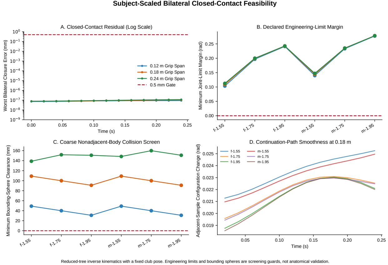
Figure 17.5: Subject-Scaled Bilateral Closed-Contact Feasibility
