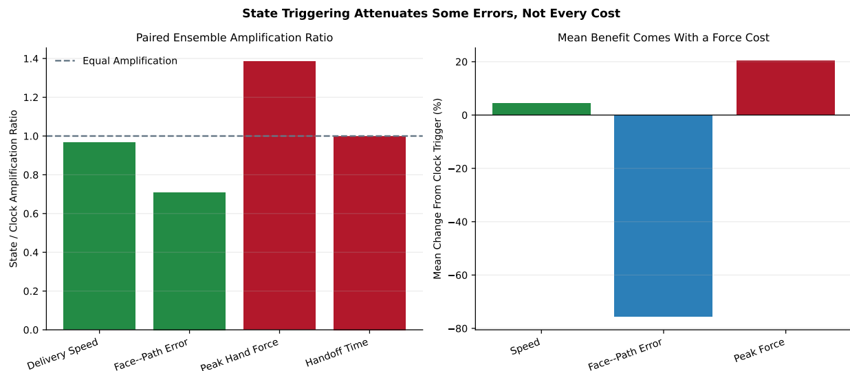
Figure 24.3: State-triggered handoff reduces speed and face/path amplification relative to clock timing but amplifies peak hand force. The right panel expresses paired mean changes as percentages so unlike units are not visually conflated.
